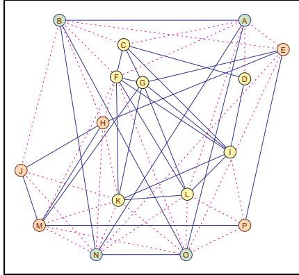
Figure 5: Gahuku-Gama Subtribes of Highland New Guinea.
