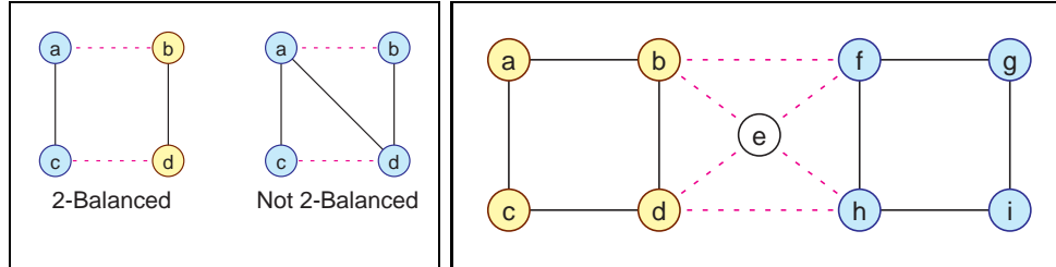
Figure 2: Two Undirected Signed Graphs (left) and A 3-Balanced Undirected Signed Graph (right).
