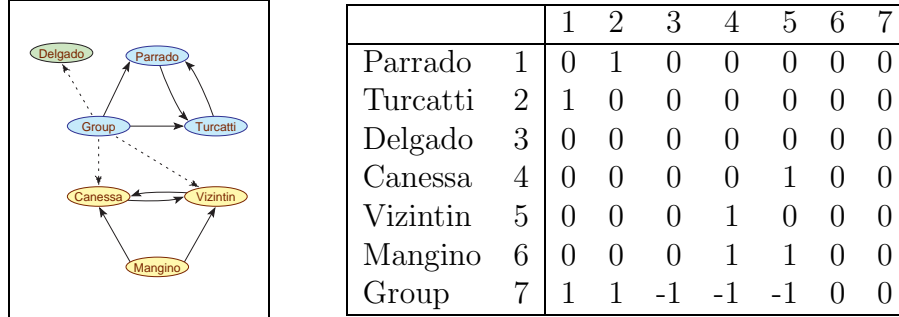
Figure 3: Directed Signed Graph for Andes Survivors.
